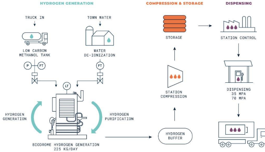
Figure 10 – Proposed CSULA Biomethanol Reformer Demonstration Process
